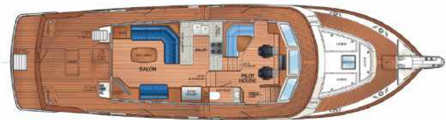
FLEMING 58 - MAIN DECK - OPTION B
