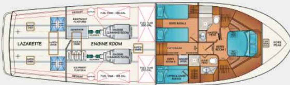
LAZARETTE | ENGINE ROOM and STANDARD ACCOMMODATION
