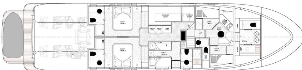
LOWER DECK
